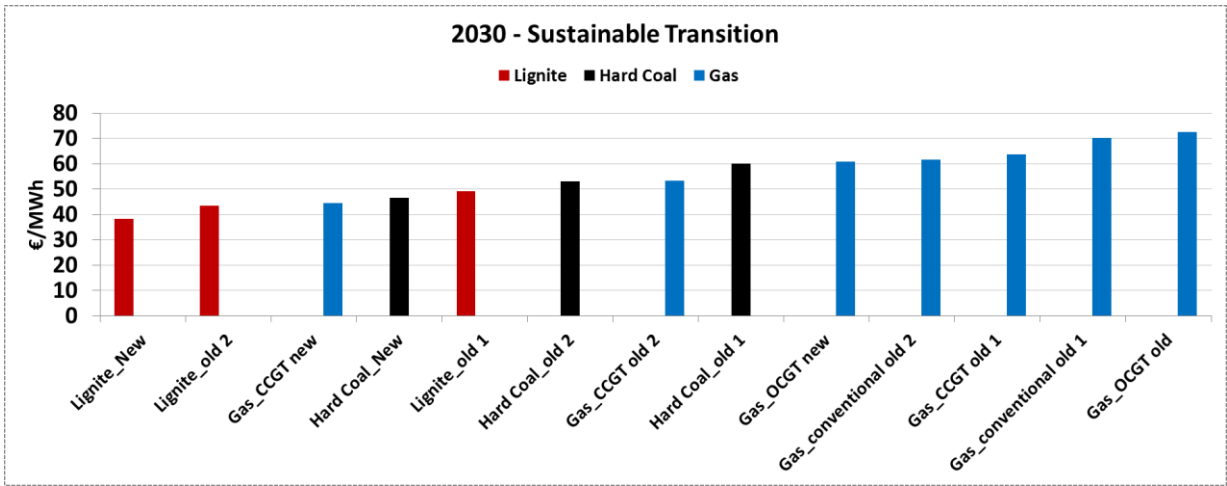
Figure 8: Sustainable Transition 2030 merit order
