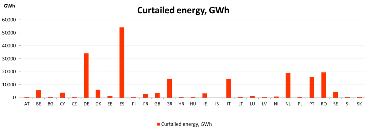
Figure 21: Curtailed Energy 2040 GCA
