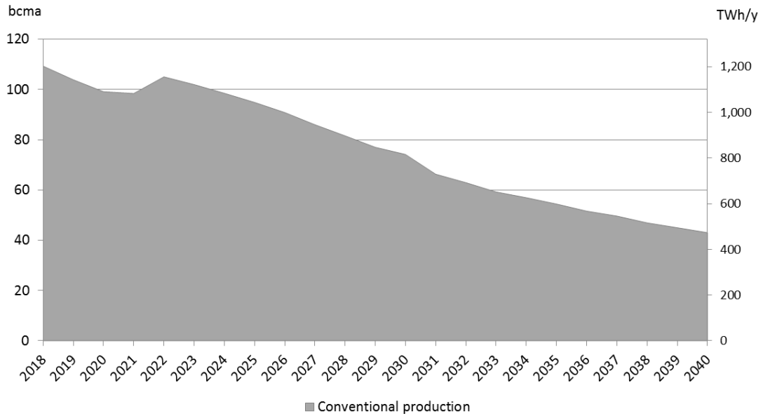
Figure 16: Potential of EU conventional production 2018-2040 (incl. Non-FID)
