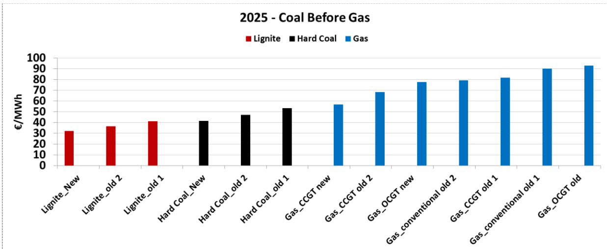
Figure 5: 2025 Coal before gas merit order
