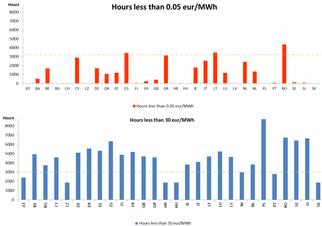
Figure 22: Number of hour's marginal price under 0.05 and 30 eur/MW 2040 GCA
