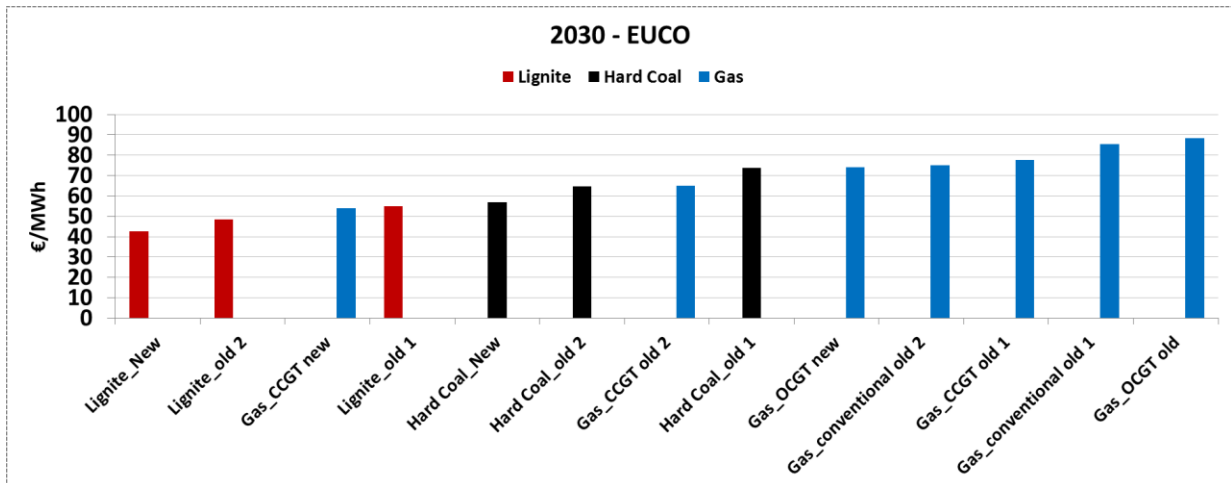
Figure 7: EUCO 2030 merit order
