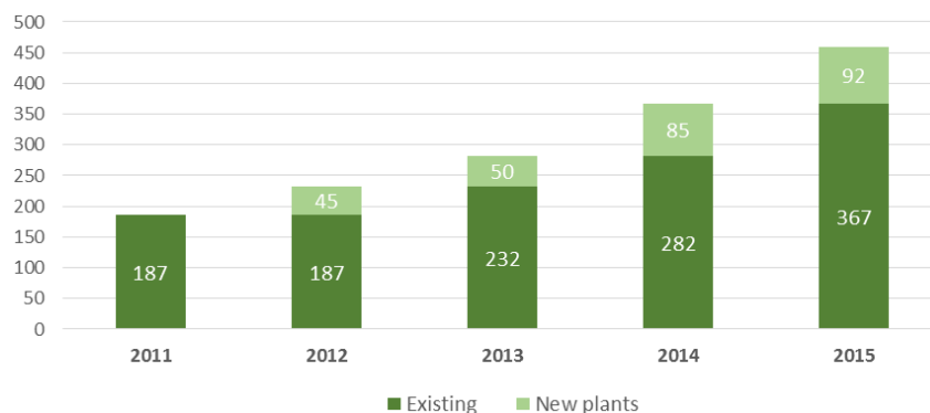
Figure 18: European biomethane plants 2015 (EBA)
