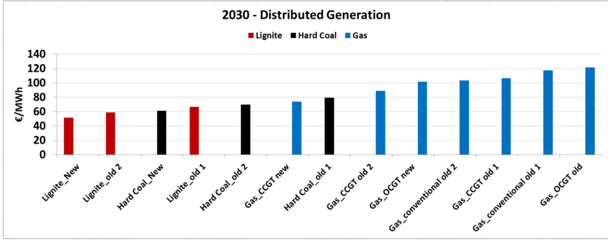
Figure 10: Distributed Generation 2030 merit order
