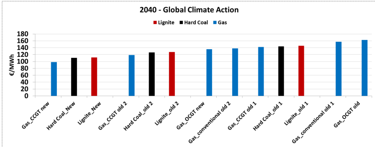
Figure 12: Global Climate Action 2040 merit order
