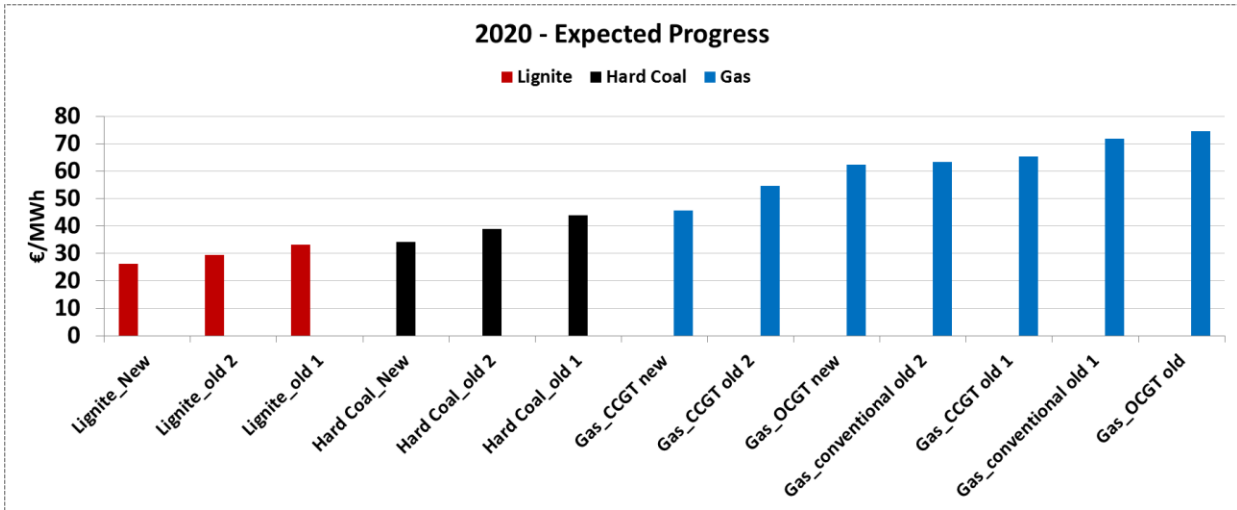
Figure 4: 2020 merit order
