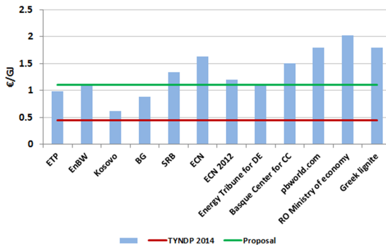
Figure 2: Lignite price
