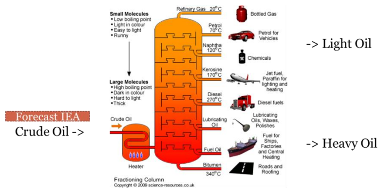
Figure 3: Crude oil conversion
