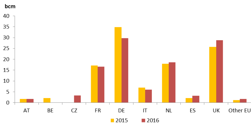
Figure 25 - Norwegian pipeline exports by destination in 2015-2016 (source BP Statistical Review 2017)
