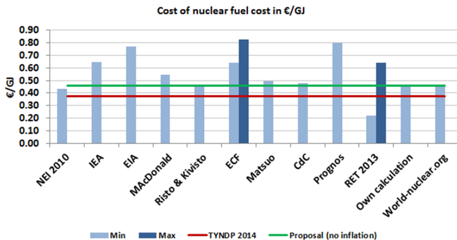
Figure 1: Nuclear price
