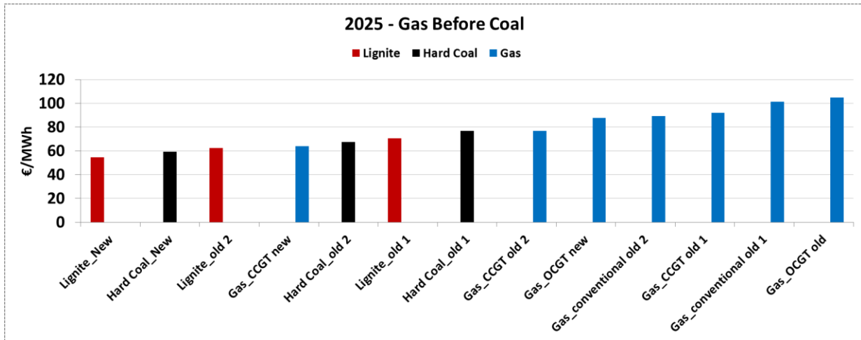
Figure 6: 2025 Gas before coal merit order
