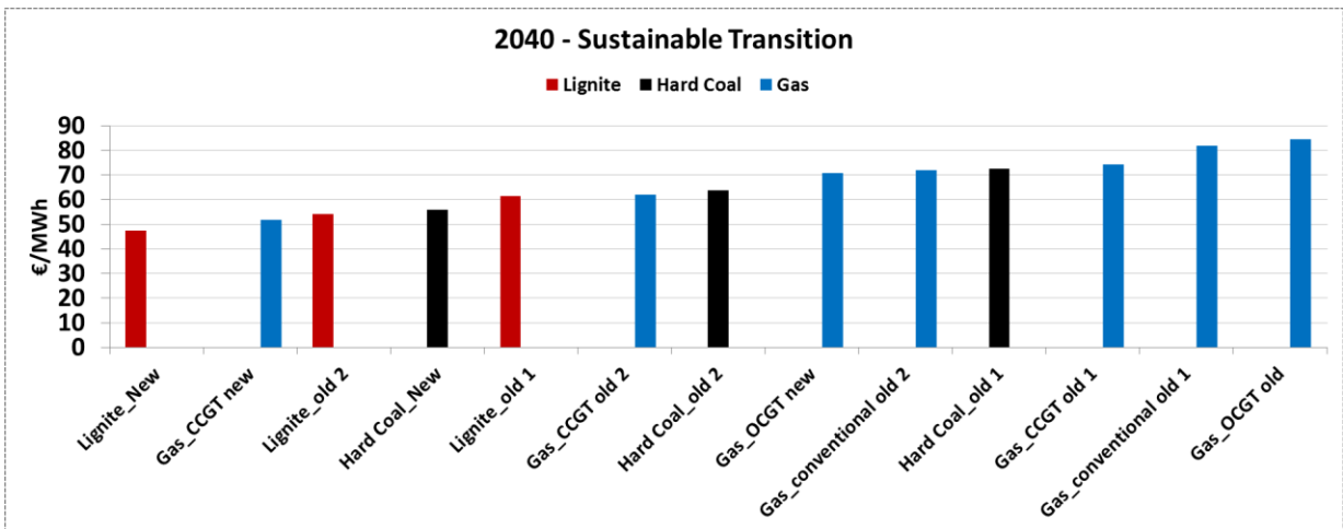
Figure 9: Sustainable Transition 2040 merit order
